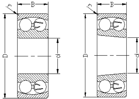
Cylindrical Bore
